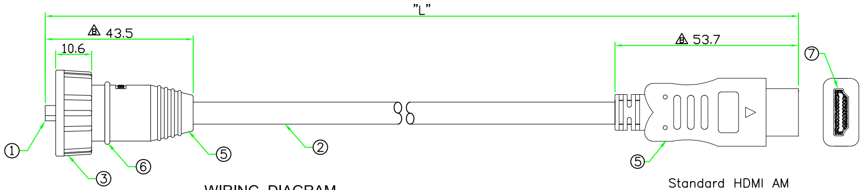
HDMI A 19M
