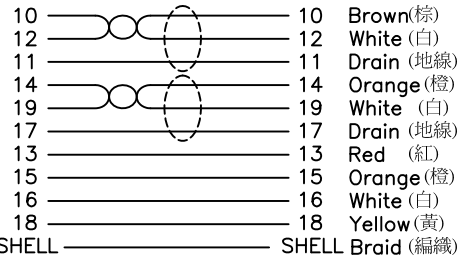
HDMI A 19M
