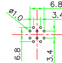
CBN-P110CPF
