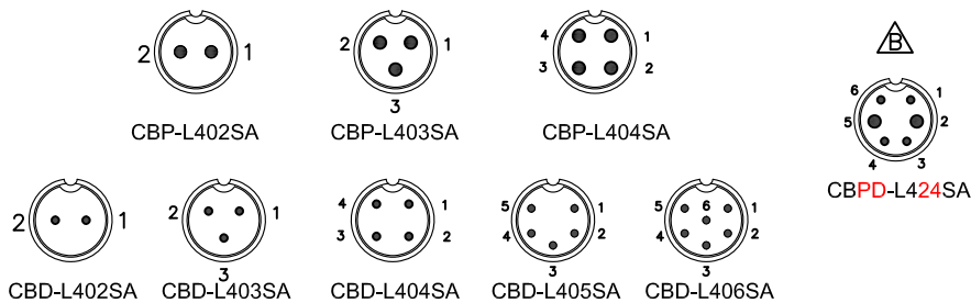
PIN ASSIGNMENT FRONT VIEW (前視圖)
