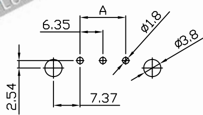
RECOMMENDED PCB LAYOUT (PCB THK=1.0~1.6)
